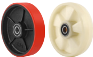
Polyurethane or Nylon Steering Wheels • Ø180 x 50
