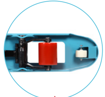
Single / Tandem load wheels
