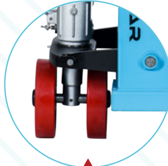
Leak-proof and reliable hydraulic pump
